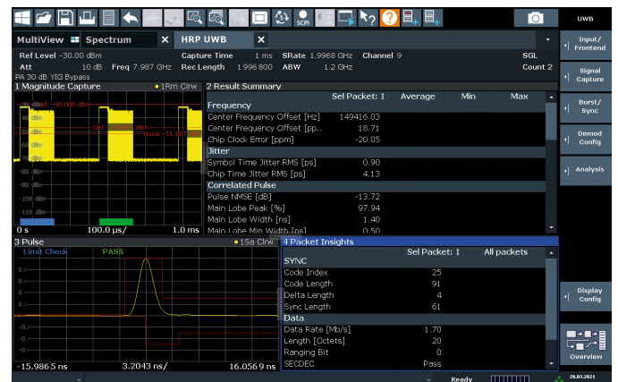
HRP UWB signal analysis with the R&S®FSW-K149 high rate pulse repetition frequency ultrawideband measurement application.
